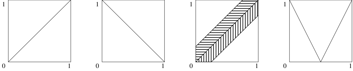
Figure 1: Various dependence prescriptions
